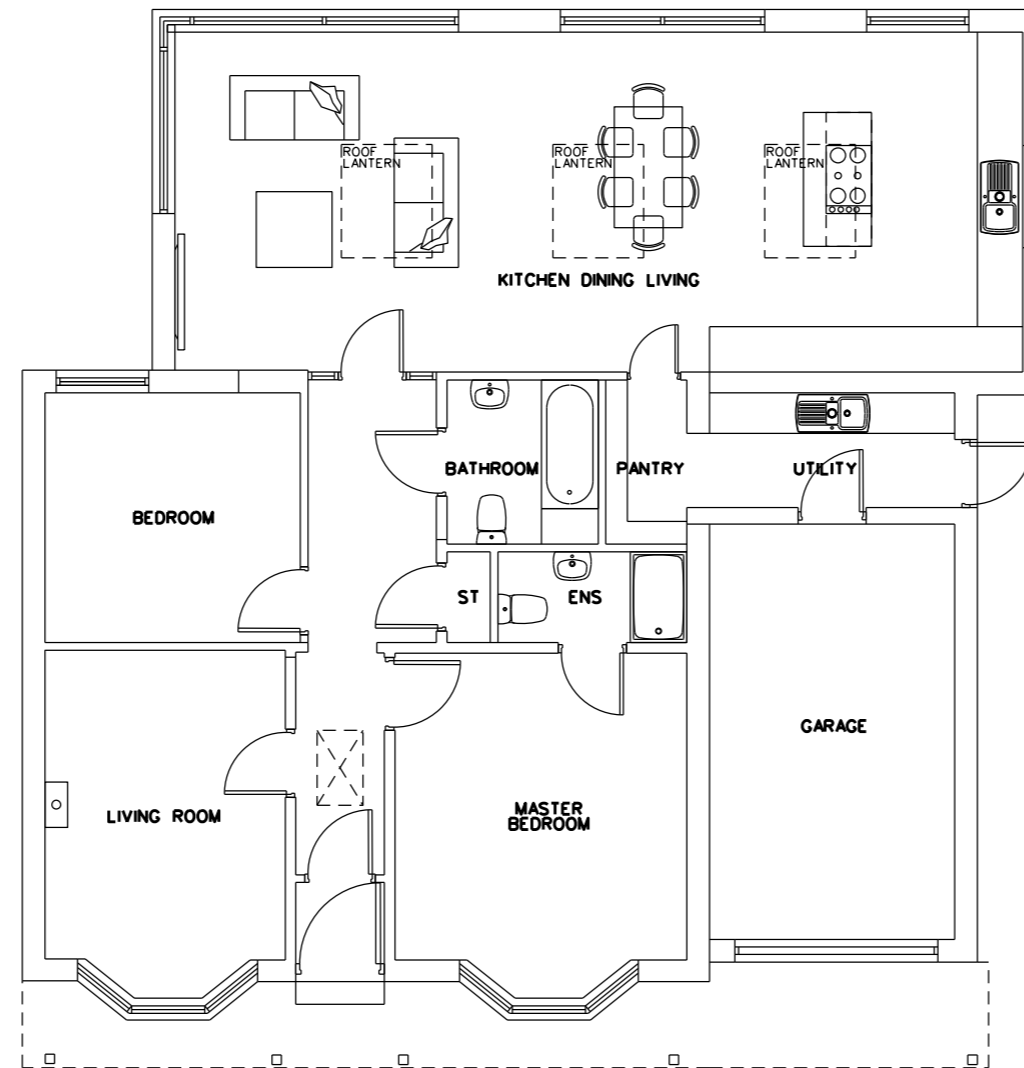
PROPOSED PLAN
